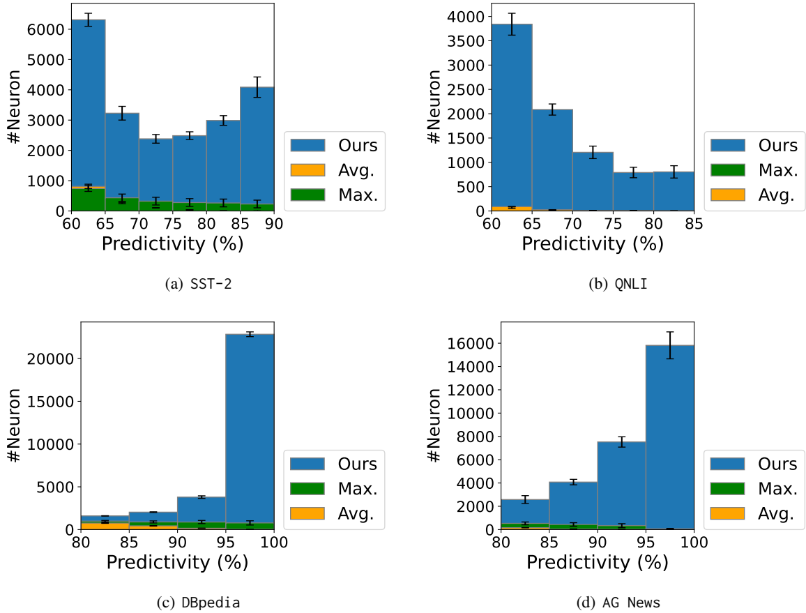
Figure 9: Histograms of predictivity for various tasks on neurons within RoBERTa BASE . Error bars indicate \pm 1 s.e.m. over 5 random trials.
