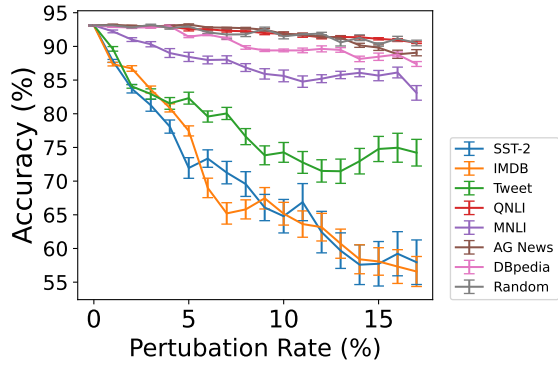
(a) On SST-2
